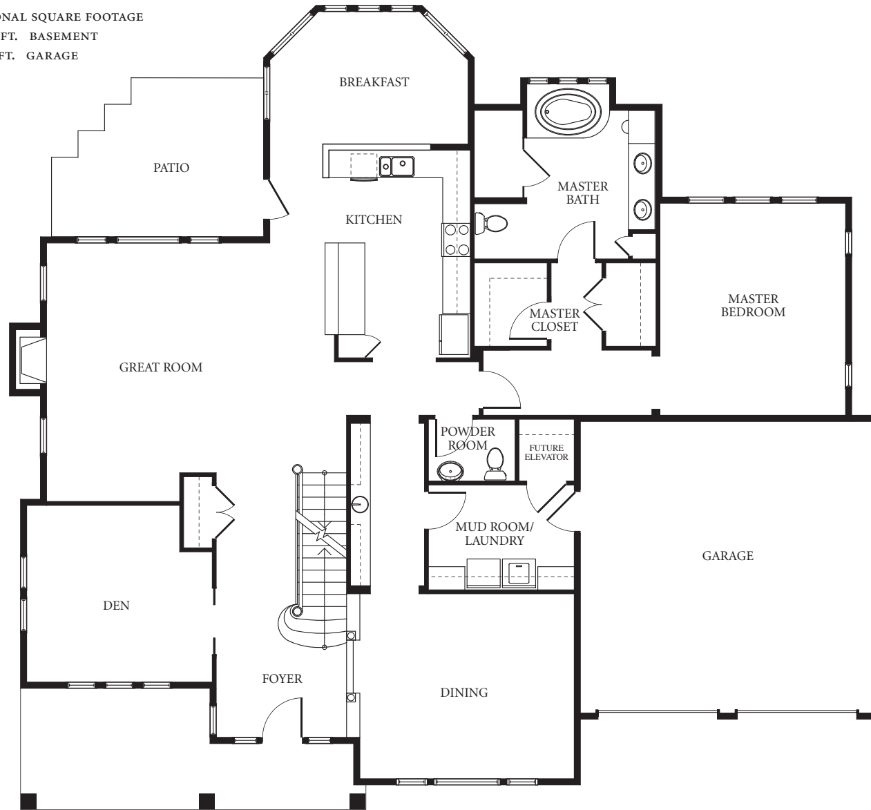
FIRST FLOOR
